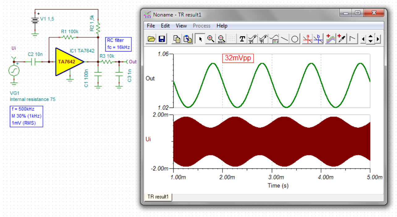
Filtered output
