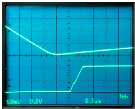
Drive Output Waveform C_L = 1 \text{ nF}
