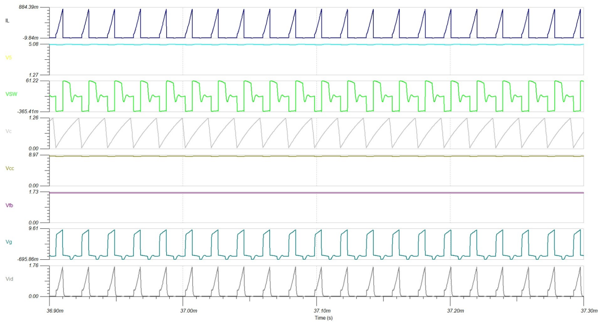
Drive Output Waveform C_L = 1 \text{ nF}
