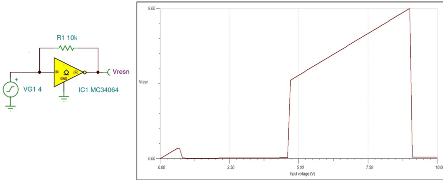
MC34064P-5G
