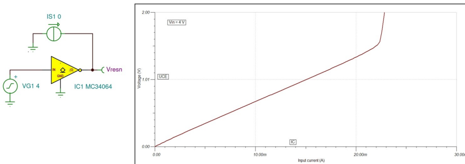
Reset Output Saturation versus Sink Current
