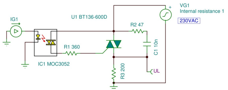
BT136-600D
